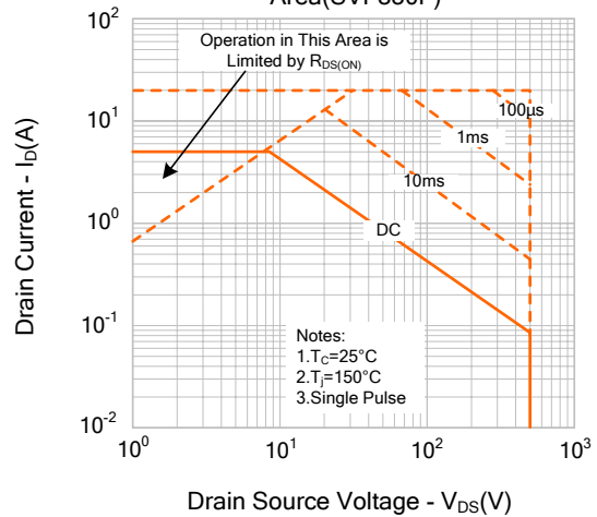
Figure 9-2. Max. Safe Operating Area(SVF830F)
